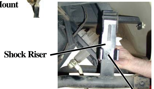
Second Shock Riser Hole 25/64"
