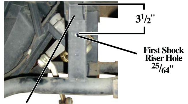
Shock Mount
